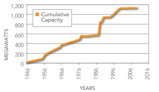
CHP GENERATING CAPACITY IN MAINE 1946-2009
