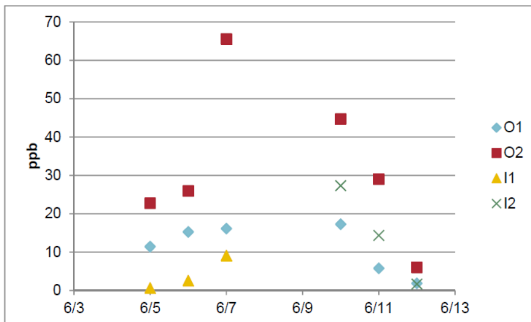
Figure 13. Average \text{NO}_x concentration values, by sample location, for the six-day study.
