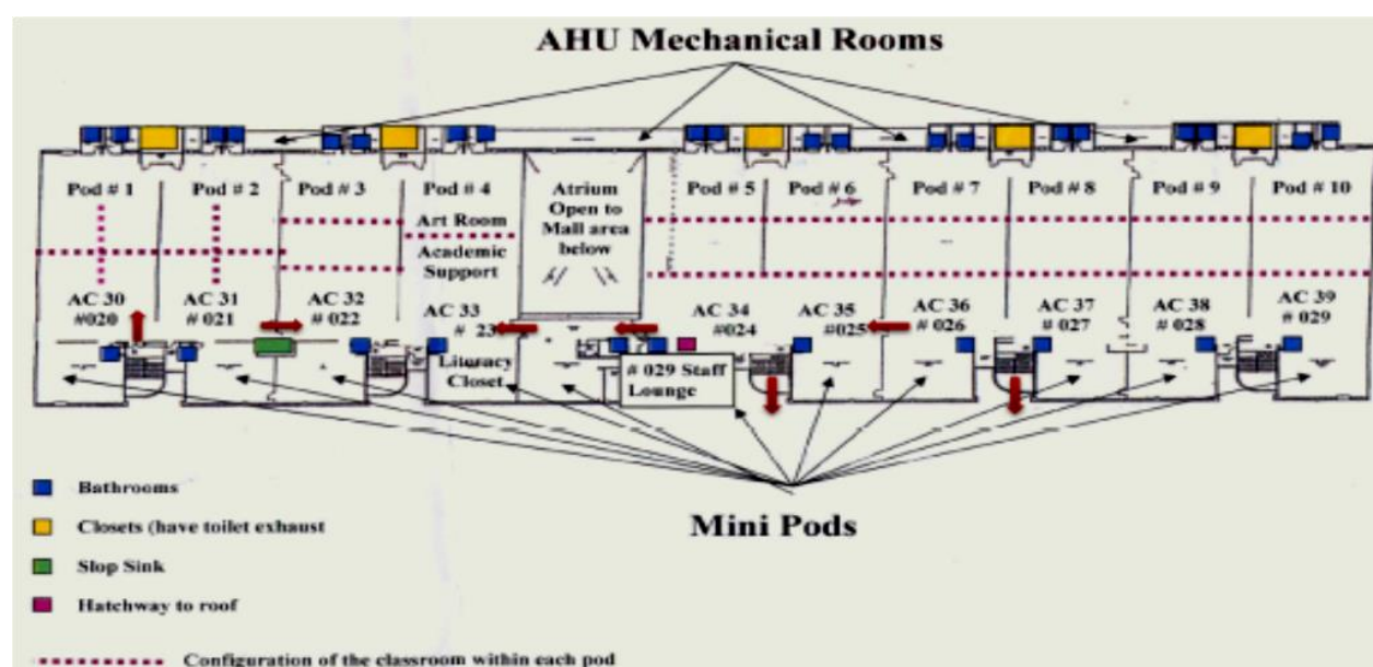
Figure 9. Air pressure mapping on third level of Building B, with direction indicated by red arrows.
