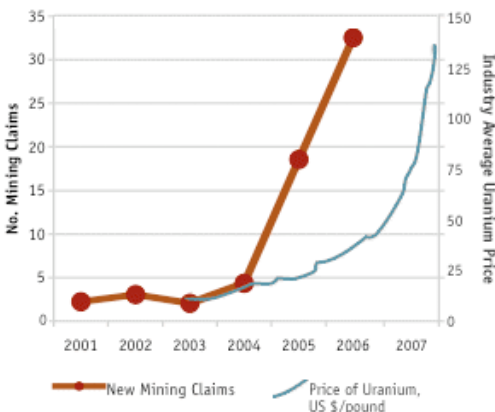
Fig 2. Mining claims in four Western states (1,000) from 2001 to 2006 overlayed with industry average uranium prices (US $/lb). Source: Bureau of Land Management (BLM Uranium). 2007. Uranium Mining Claim Activity in CO, NM, UT, and WY. Cameco (Cameco). 2007. Industry Average Uranium Spot Price.
