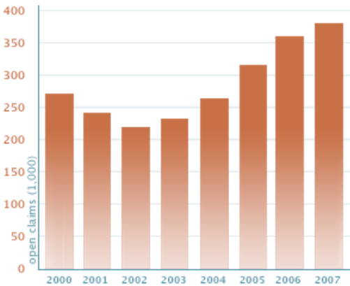
Fig 1. Active claims (1,000) from 2000 to 2007. Environmental Working Group analysis of Bureau of Land Management's LR2000 Database, July 2007 download.
