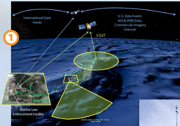
(above) Nested concept of operations showing data flow. Two PGST towers were employed during the MDA demonstration, one on Koror (due to topography, full 360° coverage was not available), and one on Kayangel (top middle full yellow circle). (right) Shore-based tower on Kayangel with radar, sensors, and satellite communications systems.
