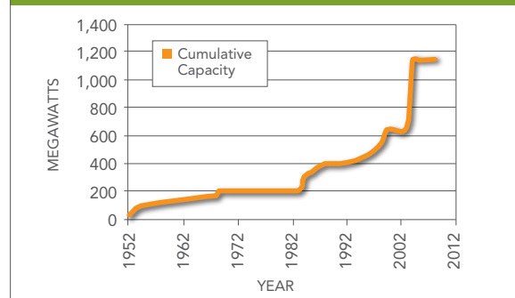
CHP GENERATING CAPACITY IN SOUTH CAROLINA 1952-2008
