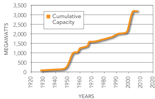
CHP GENERATING CAPACITY IN ALABAMA 1928-2007
